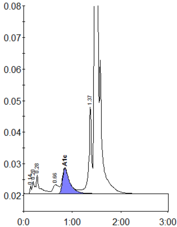
Peak table - ID: 10173470
