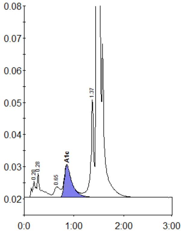
Peak table - ID: 10142256
