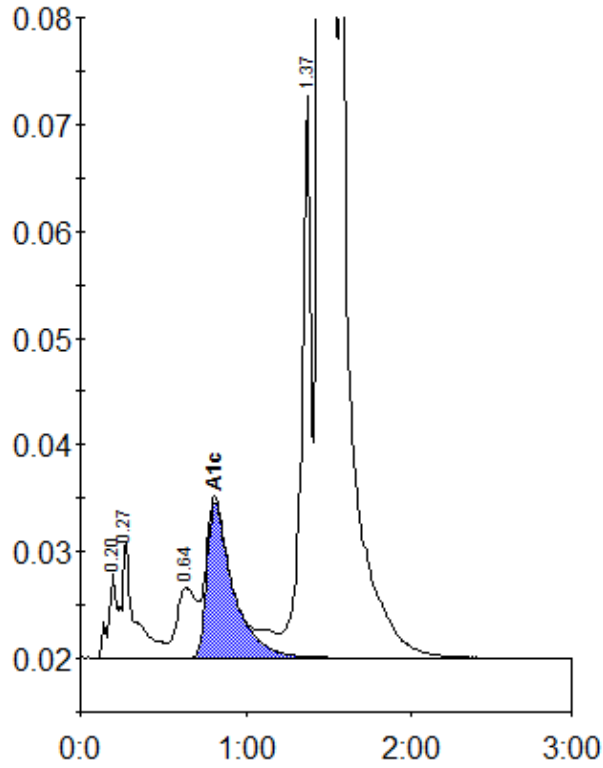
Peak table - ID: 10229677
