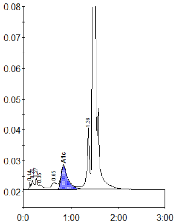
Peak table - ID: 10161163
