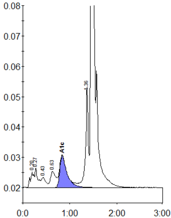
Peak table - ID: 10176748
