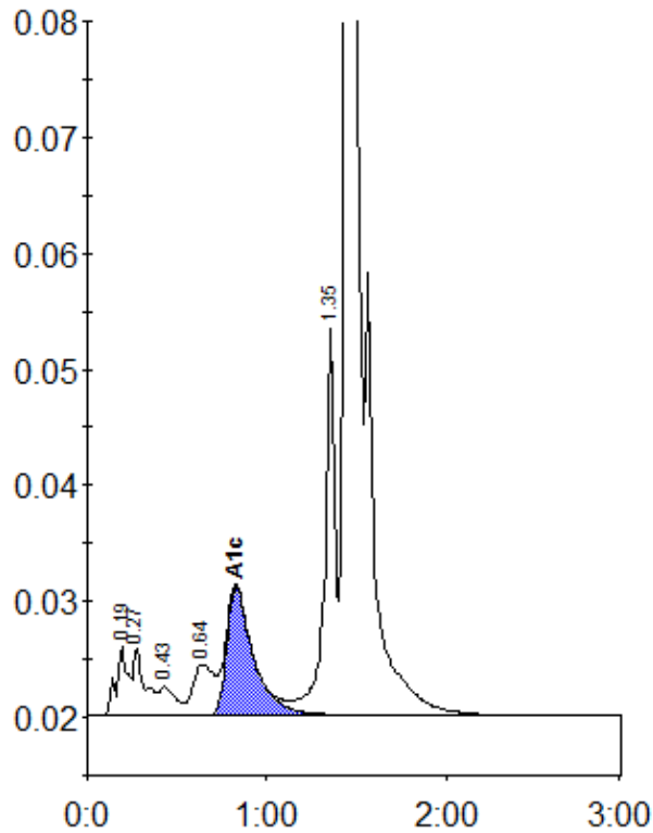
Peak table - ID: 10132151
