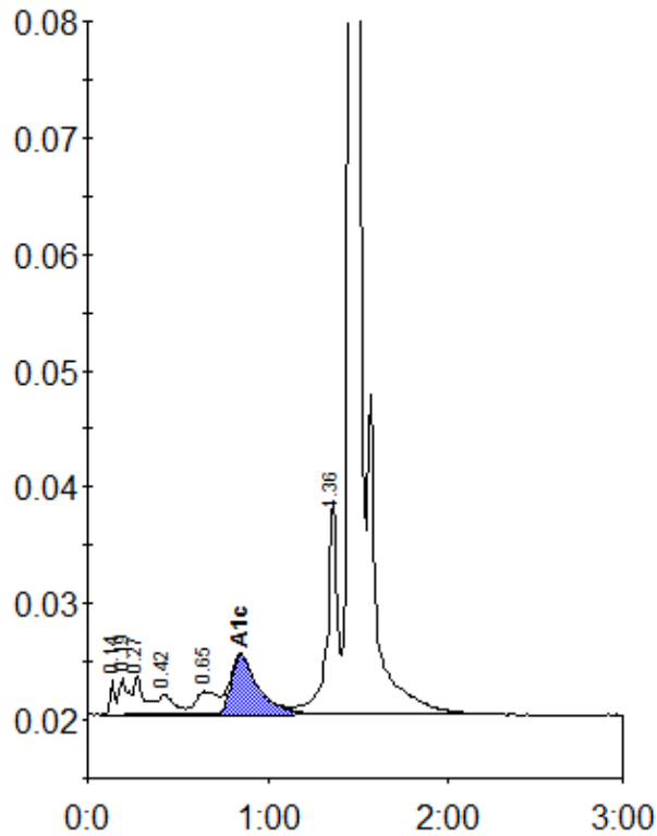
Peak table - ID: 10169791
