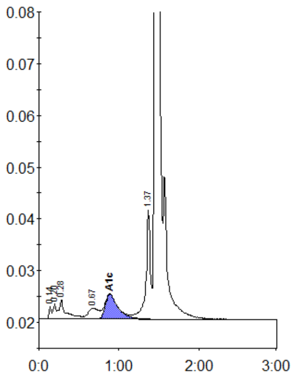
Peak table - ID: 10145117
