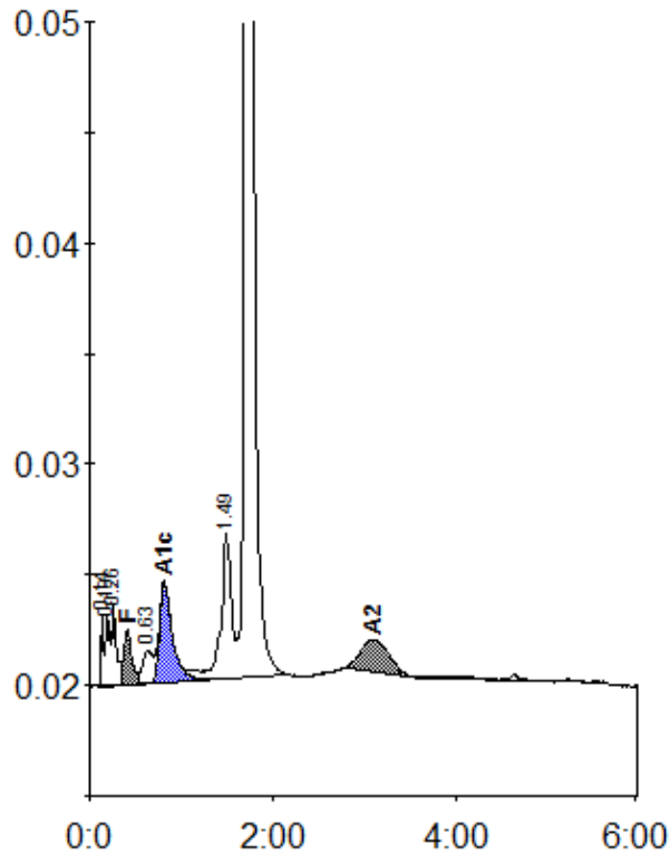
Peak table - ID: 10132398
