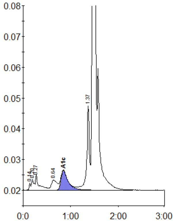
Peak table - ID: 10141489
