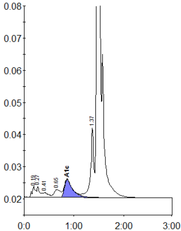
Peak table - ID: 10141661
