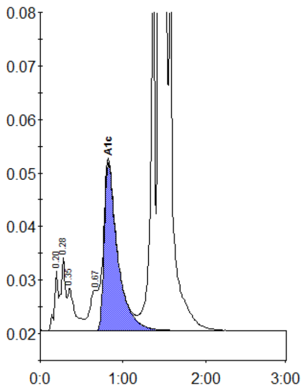
Peak table - ID: 10179033
