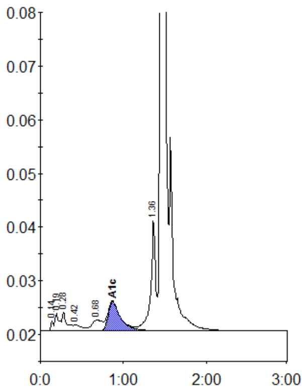
Peak table - ID: 10131814
