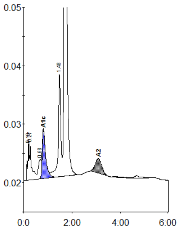
Peak table - ID: 10176801
