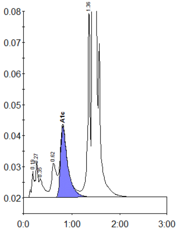
Peak table - ID: 10145670
