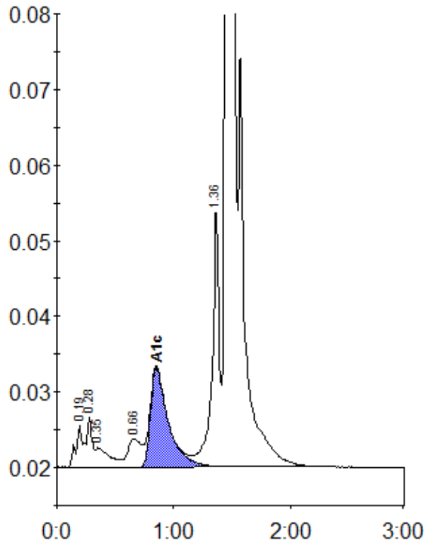
Peak table - ID: 10154173
