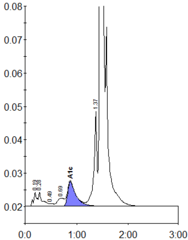
Peak table - ID: 10145633
