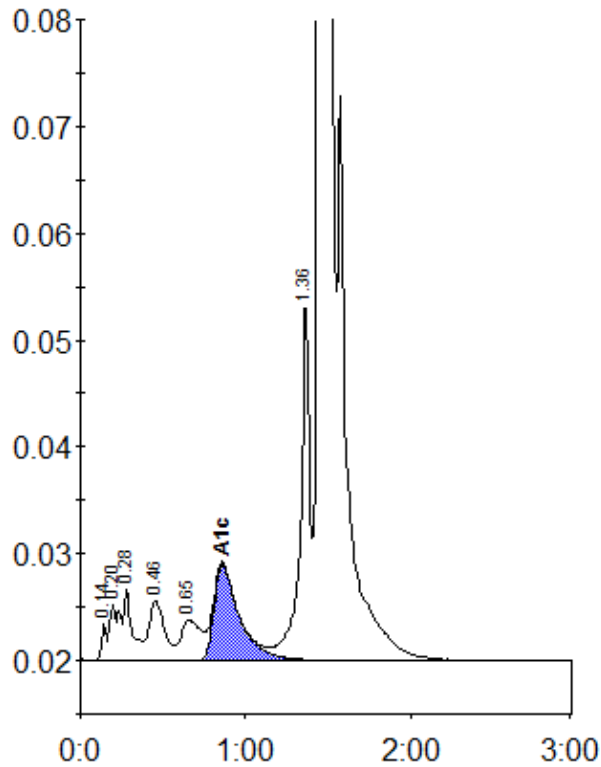
Peak table - ID: 10122185
