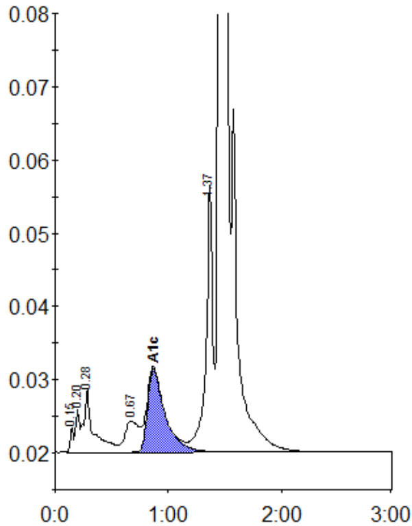
Peak table - ID: 10176671
