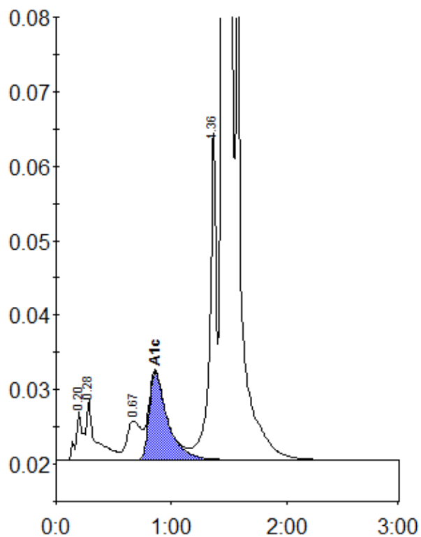
Peak table - ID: 10130284
