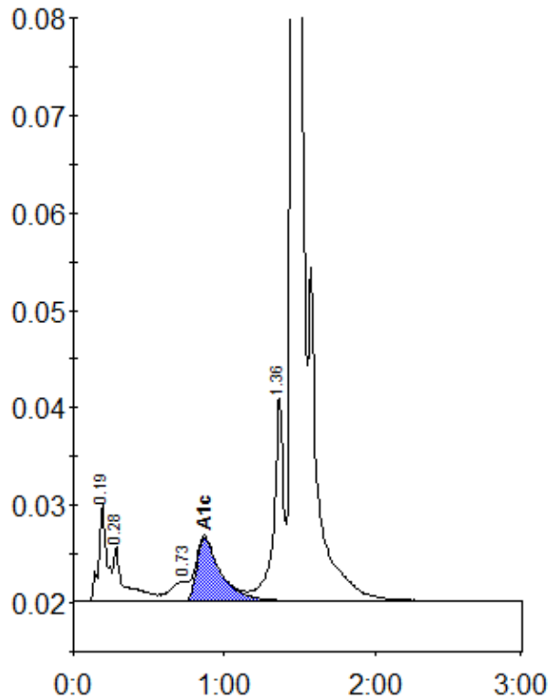
Peak table - ID: 10175263
