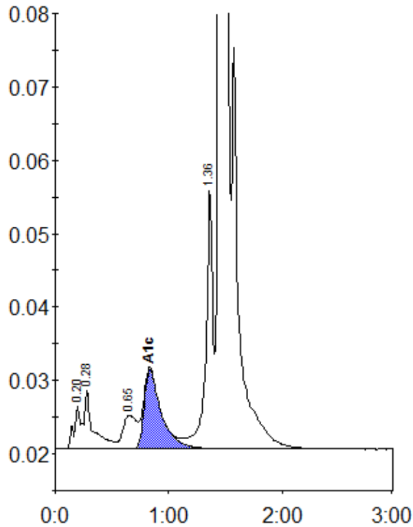
Peak table - ID: 10055117
