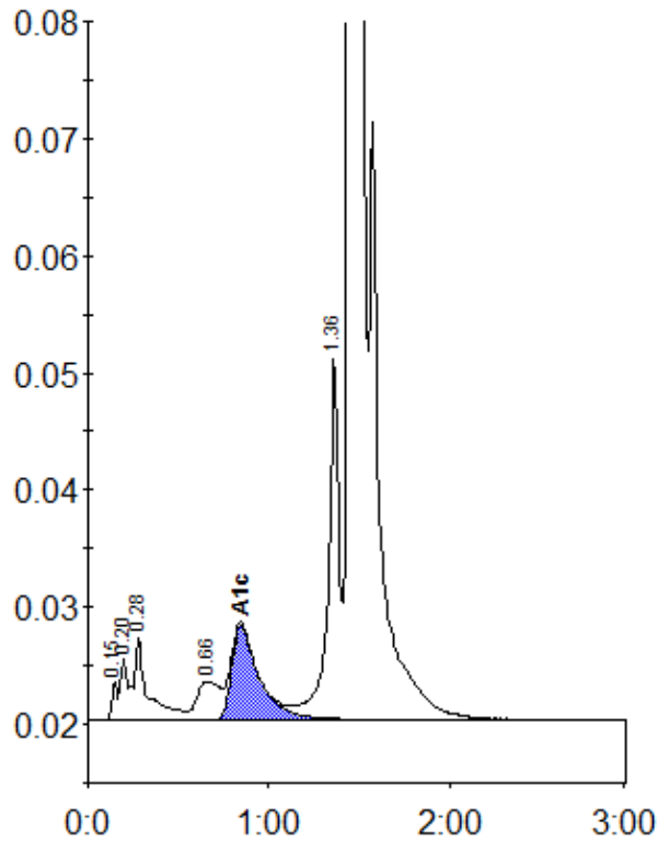
Peak table - ID: 0090937
