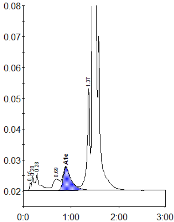
Peak table - ID: 10156024
