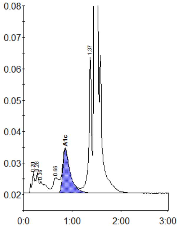
Peak table - ID: 10148286
