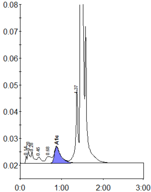
Peak table - ID: 10043541
