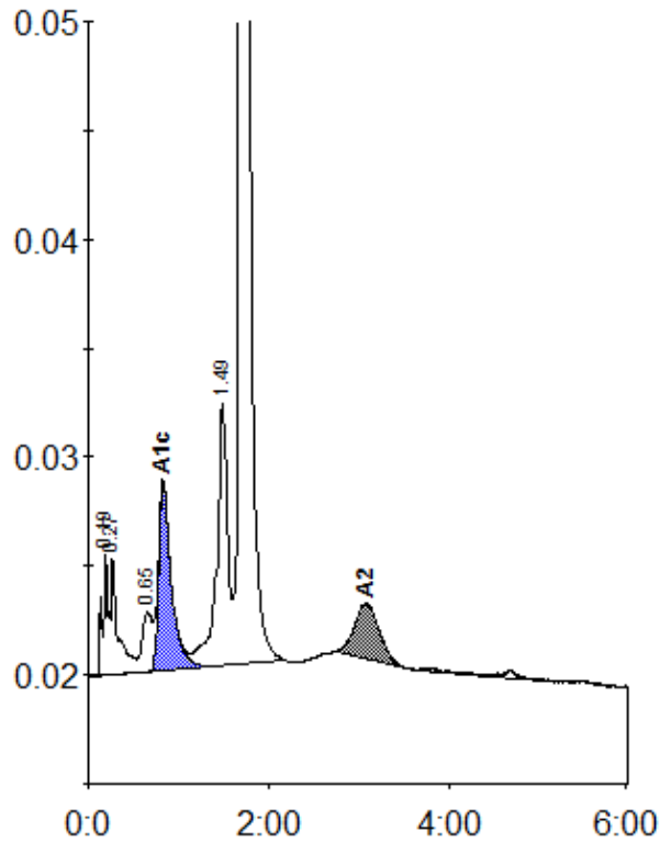
Peak table - ID: 10078849
