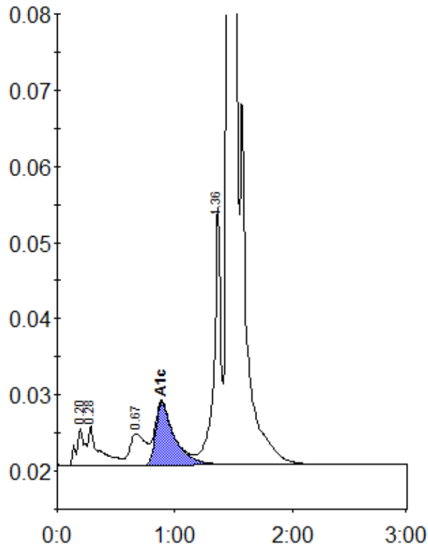
Peak table - ID: 10055297
