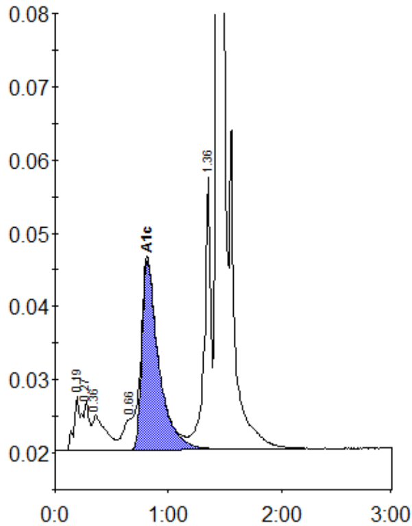
Peak table - ID: 10154417
