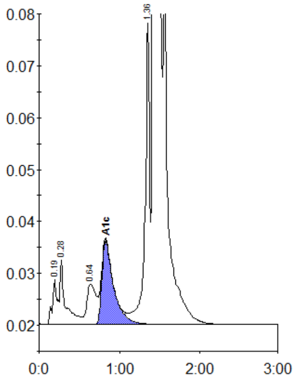
Peak table - ID: 10147610
