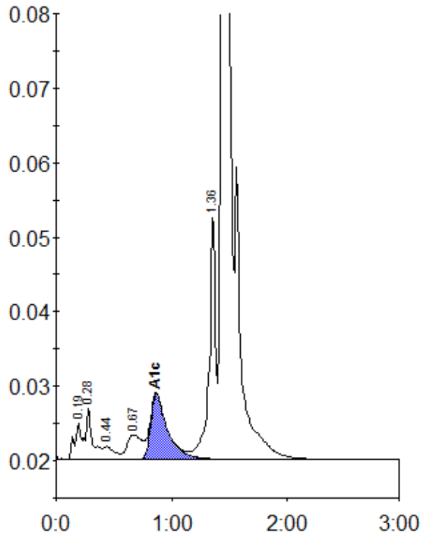
Peak table - ID: 10147186
