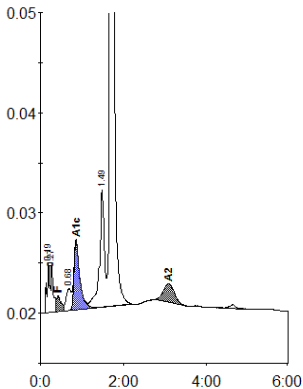
Peak table - ID: 10147576
