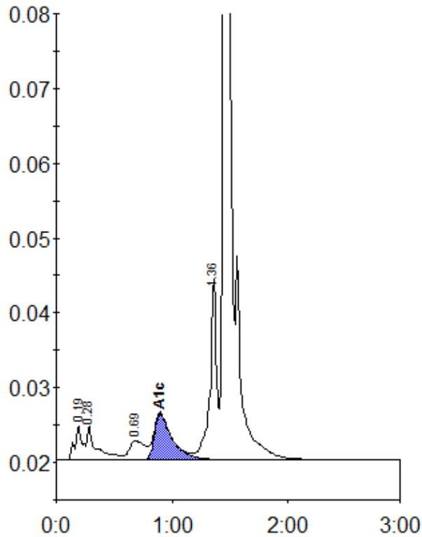
Peak table - ID: 10147565
