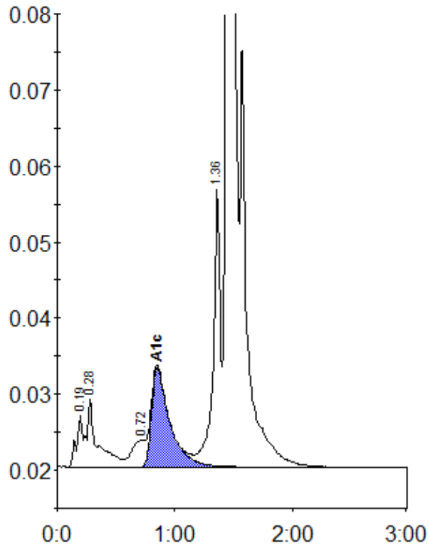
Peak table - ID: 10062082
