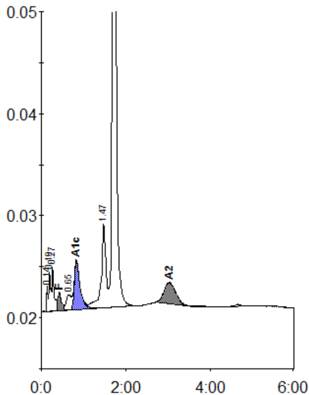
Peak table - ID: 10127275
