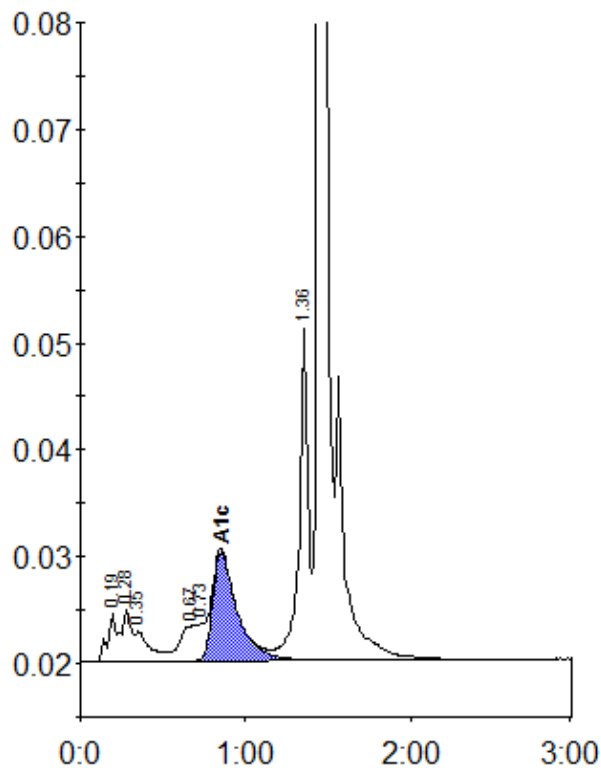
Peak table - ID: 10055486
