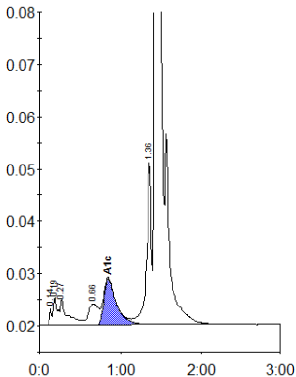
Peak table - ID: 10047541
