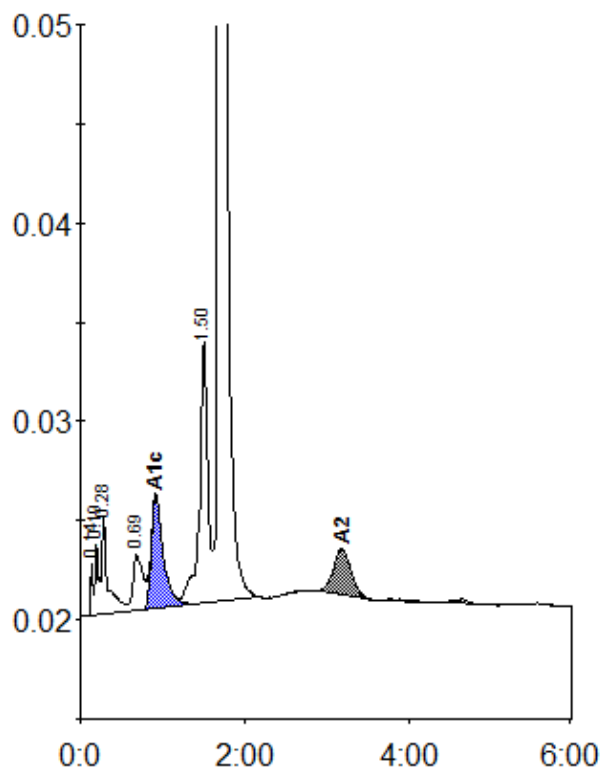
Peak table - ID: 10076548
