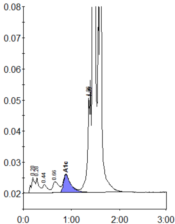
Peak table - ID: 10054821
