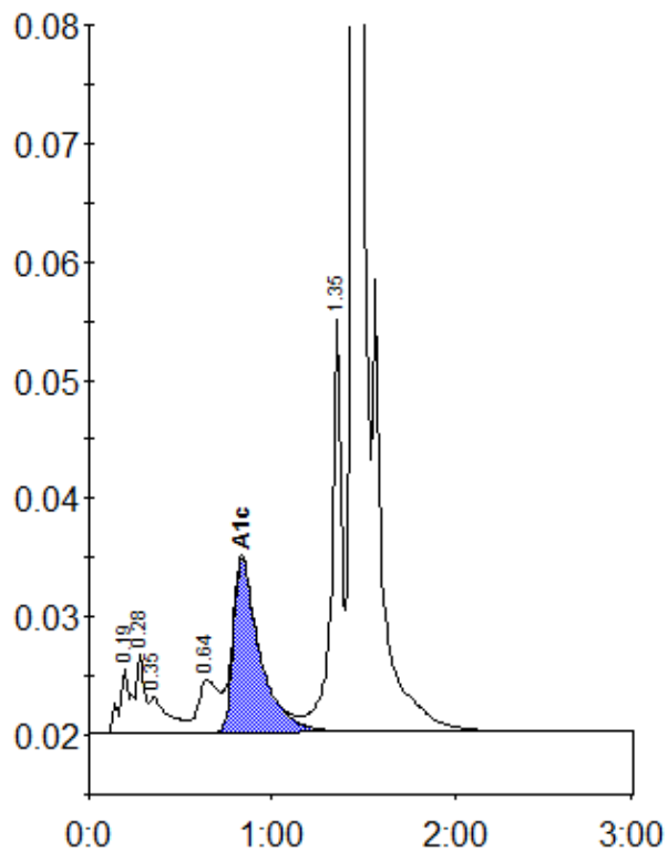
Peak table - ID: 10068511
