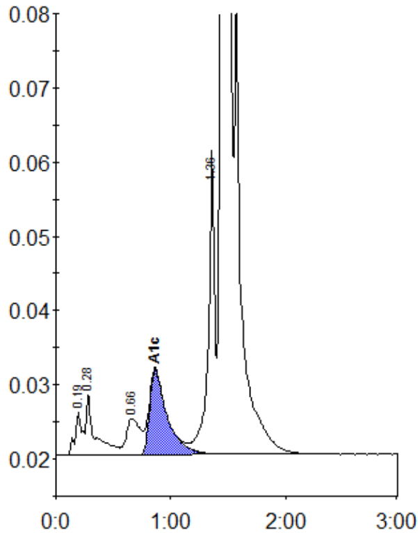
Peak table - ID: 16370500
