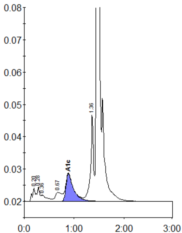
Peak table - ID: 10062893
