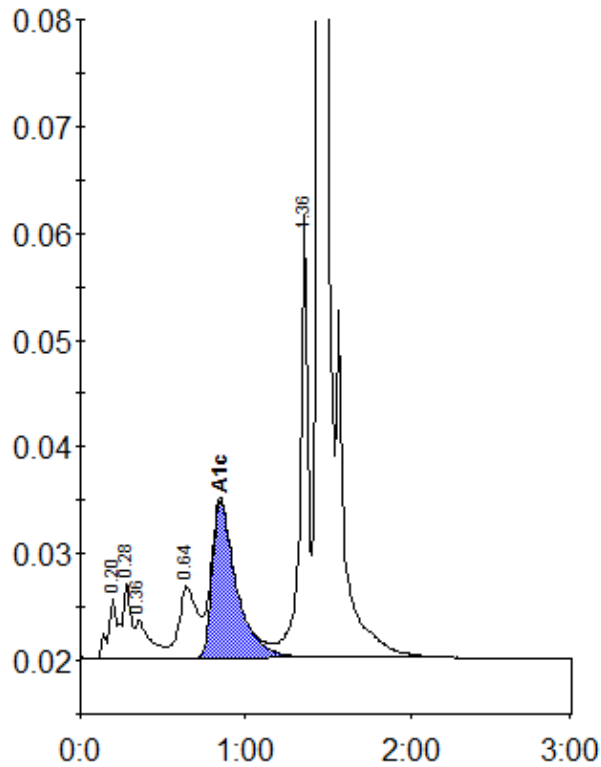
Peak table - ID: 10091412
