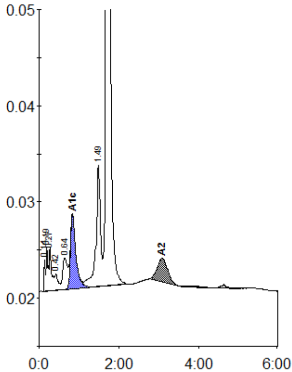
Peak table - ID: 10101682
