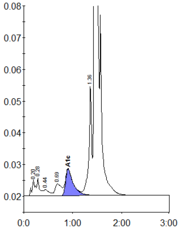
Peak table - ID: 10075241
