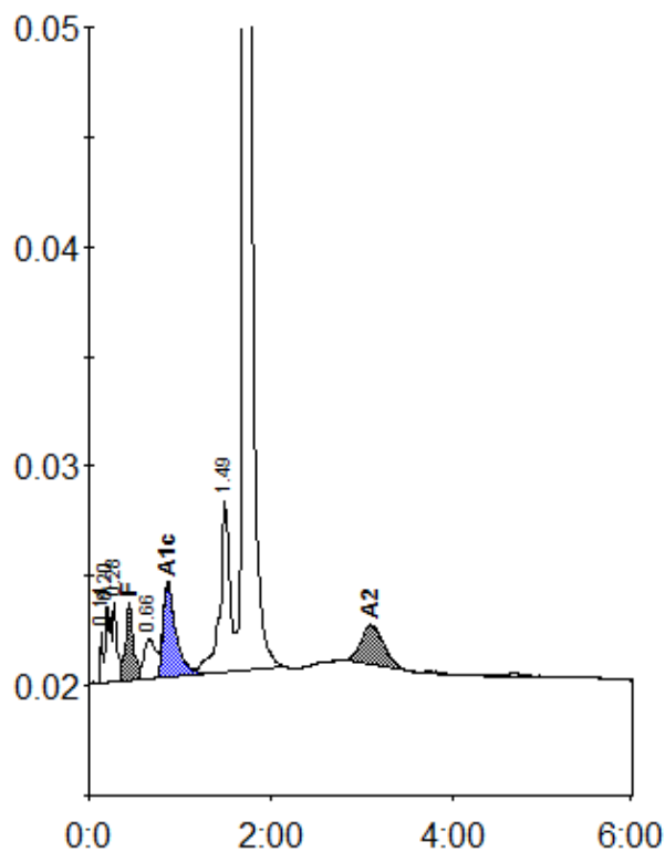
Peak table - ID: 10054591
