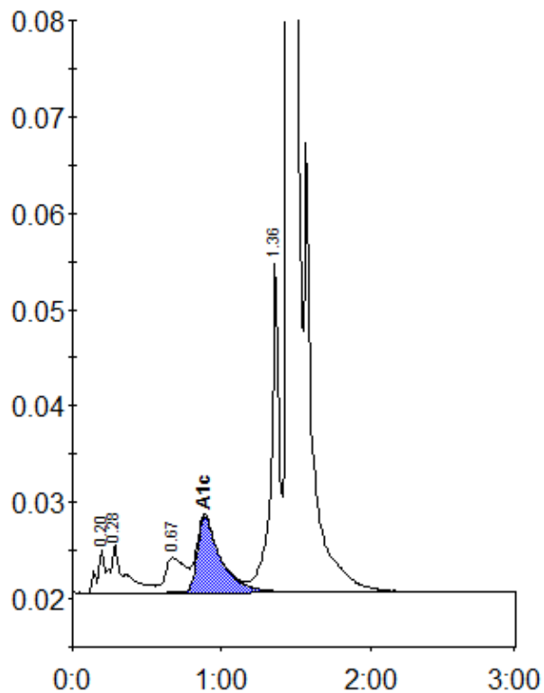
Peak table - ID: 10109115
