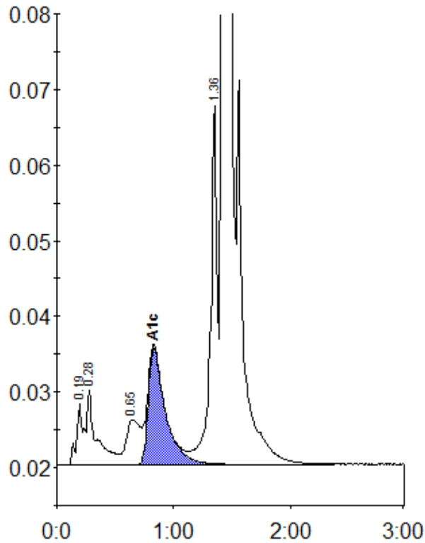
Peak table - ID: 10109307
