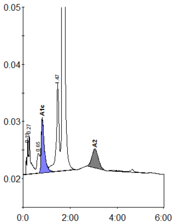
Peak table - ID: 10080340
