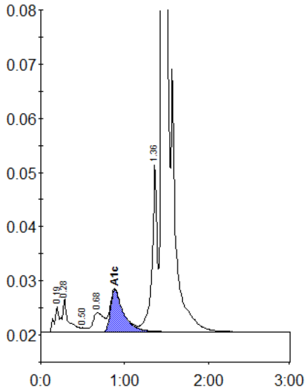
Peak table - ID: 10094380
