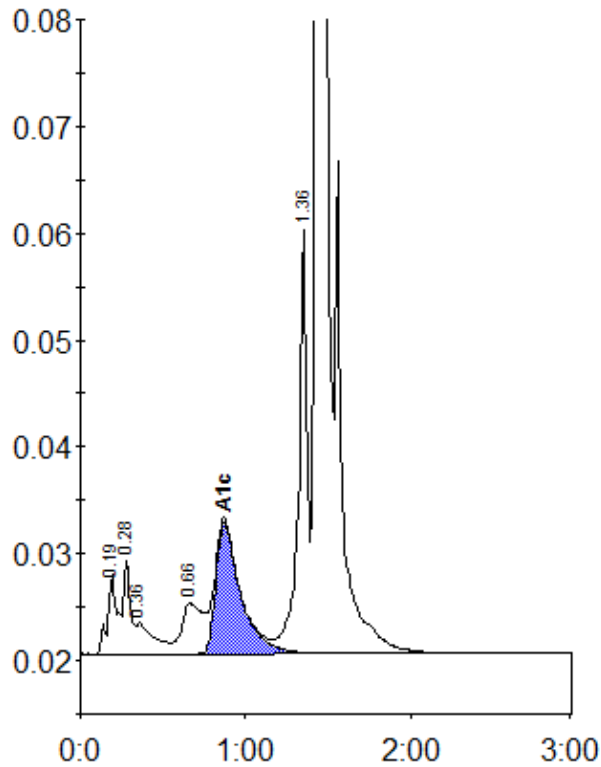
Peak table - ID: 10102919
